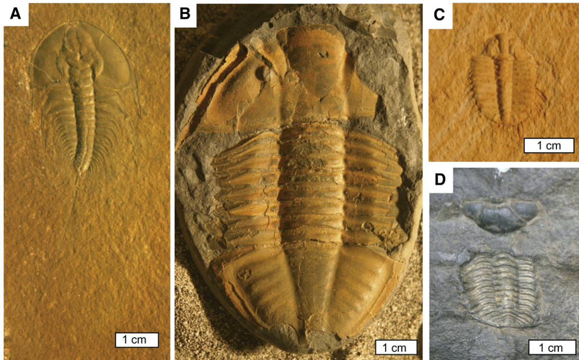
Fig. 4. Exceptional preservation of fossil trilobites: A, Olenellus sp. aff. O. gilberti complete with pleural spines and flexuous telson, oxidized internal mold, from Eager Formation (late Early Cambrian) near Cranbrook, British Columbia, Canada; B, Hoekaspis matacensis molt with displaced free cheeks, oxidized internal mold in siderite nodule, from San Luis Ocuri Formation (lower Dapingian, early Middle Ordovician) near Camargo, Bolivia; C, Sinespinaspis markhami molt without free cheeks, oxidized internal mold, from Cotton Beds (upper Telychian, late Early Silurian) near Forbes, N.S.W., Australia; D, Trimerocephalus mastopthalmus molt of Salterian mode (with reversed cephalon), compression in shale, from Ostracod Slate (late Frasnian, mid-Late Devonian) near Newton Abbott, England. Specimen numbers are F112142A (A), F108966 (B), F113639A (C), and P13132 (D), in Condon Collection, Museum of Natural and Cultural History, University of Oregon, Eugene (A–C) and Natural History Museum, Kensington, London (D).
